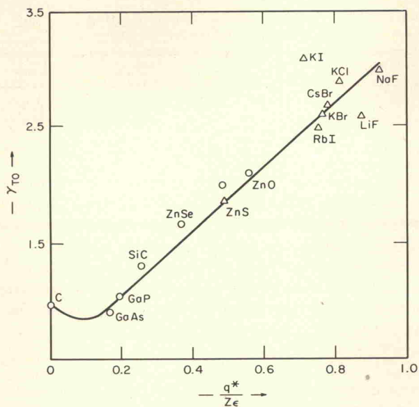
FIG. 3. Transverse-optic mode-Grüneisen parameter at \bar{k} \approx 0 vs the effective charge per electron for a number of diatomic crystals. Circles represent Raman and triangles infrared measurements. Sources of data are as follows: KI, RbI, present study; GaAs, unpublished; rest from Refs. 1-4.
